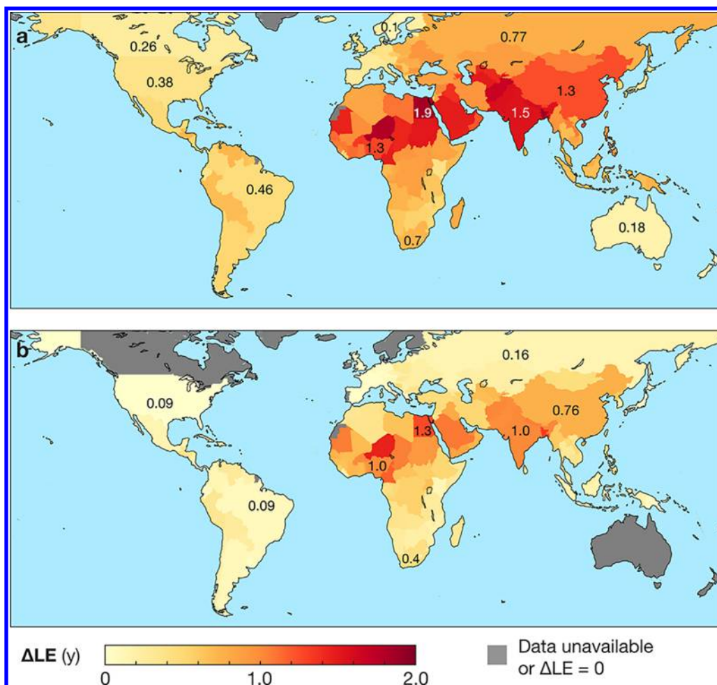
Figure 3. Global maps of the life expectancy decrement \Delta\text{LE} from \text{PM}_{2.5} . Panel a shows baseline \Delta\text{LE} for year-2016 concentrations (global population-weighted mean and median of 1.03 and 1.22 years, respectively). Panel b shows hypothetical gains in life expectancy for an alternative exposure distribution where concentrations are limited to a maximum of 10 \mu\text{g m}^{-3} , the WHO air quality guideline concentration (global-average \Delta\text{LE} of \sim 0.59 year). See also Table S2.
