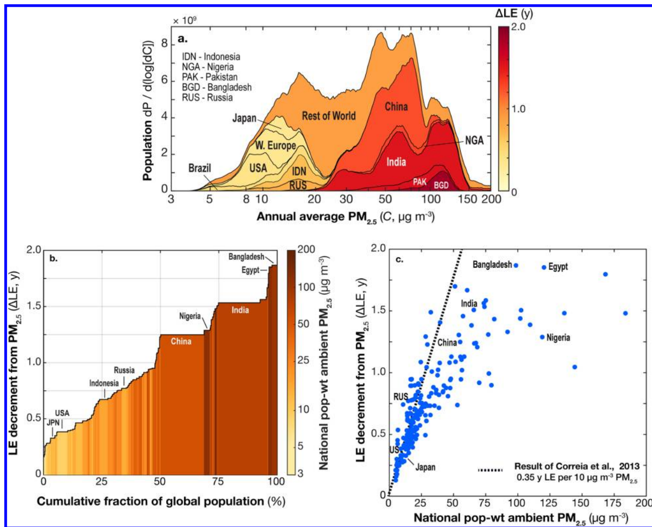
Figure 2. Relationship among the global distribution of ΔLE, the life expectancy decrement from PM 2.5 , and global PM 2.5 concentrations C. ΔLE is generally higher in countries with higher PM 2.5 levels. (a) Global distribution of population with respect to annual-average PM 2.5 for year 2016. Plotted data reflect local smoothing of bin-width-normalized distributions computed over 400 logarithmically spaced bins: equal-sized plotted areas reflect equal populations. Each country is colored proportionally to the ΔLE from PM 2.5 exposure. (b) Cumulative distribution of ΔLE over the global population. The global population-weighted median value for ΔLE is 1.22 years, corresponding to conditions in China. Shading for each country shows the national population-weighted mean PM 2.5 , illustrating how ΔLE has a strong but imperfect association with PM 2.5 . (c) National decrements in ΔLE vs PM 2.5 . Owing to the supralinear concentration–response relationship of mortality with PM 2.5 , the slope of this distribution is higher for countries with lower average PM 2.5 concentrations.
