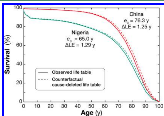
Figure 1. Example survival curves for observed life tables (solid lines) and simulated cause-deleted life tables (dashed lines) where ambient PM_{2.5} exposure is eliminated as a mortality risk factor. Life expectancy e_0 can be visualized as the integral of the survival curve over the age spectrum. Life expectancy for the counterfactual case is increased after removing PM_{2.5} as a mortality risk. For a given country, the reduction in life expectancy attributed to PM_{2.5} ( \Delta LE ) relative to a counterfactual scenario with no excess mortality risk from PM_{2.5} can be visualized as the area between the solid and dashed curves.
